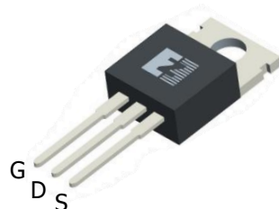
TO-220
